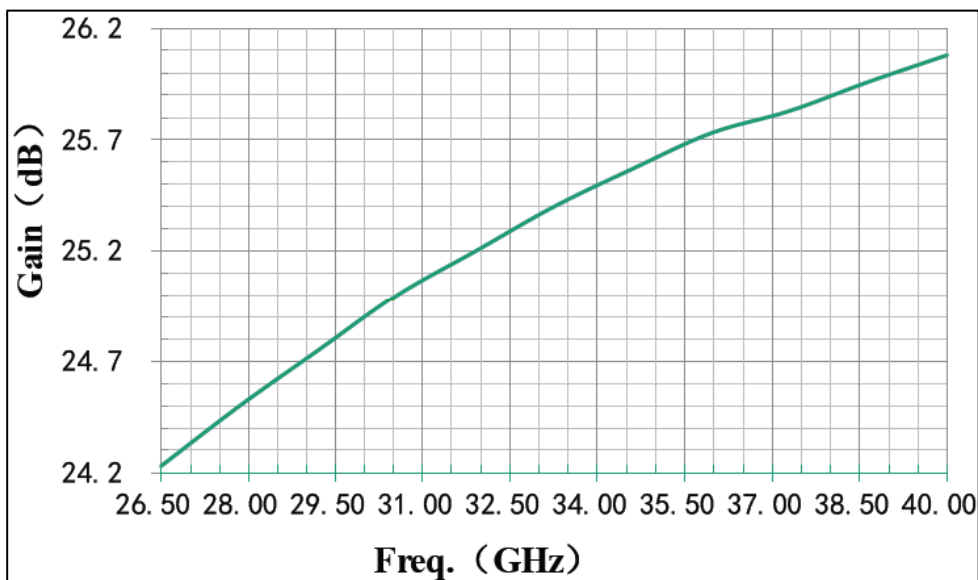
Gain
