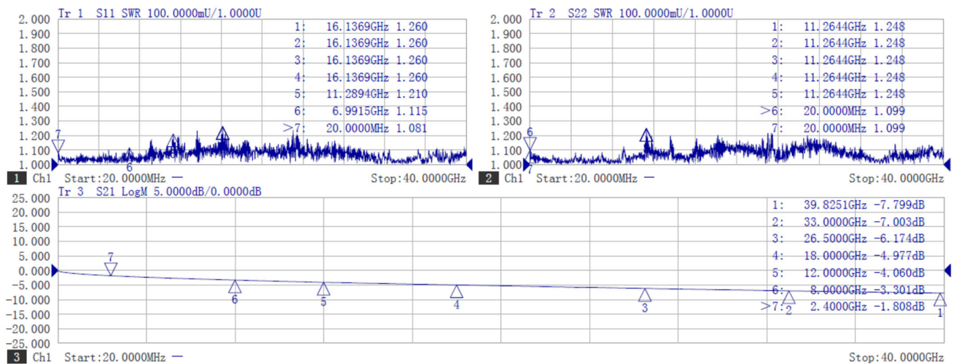
2.92mm(M)-2.92mm(F) 2.2M
