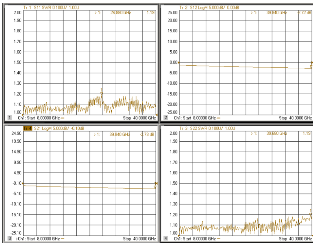
2.4mm(M)-2.92mm(M) 1M
