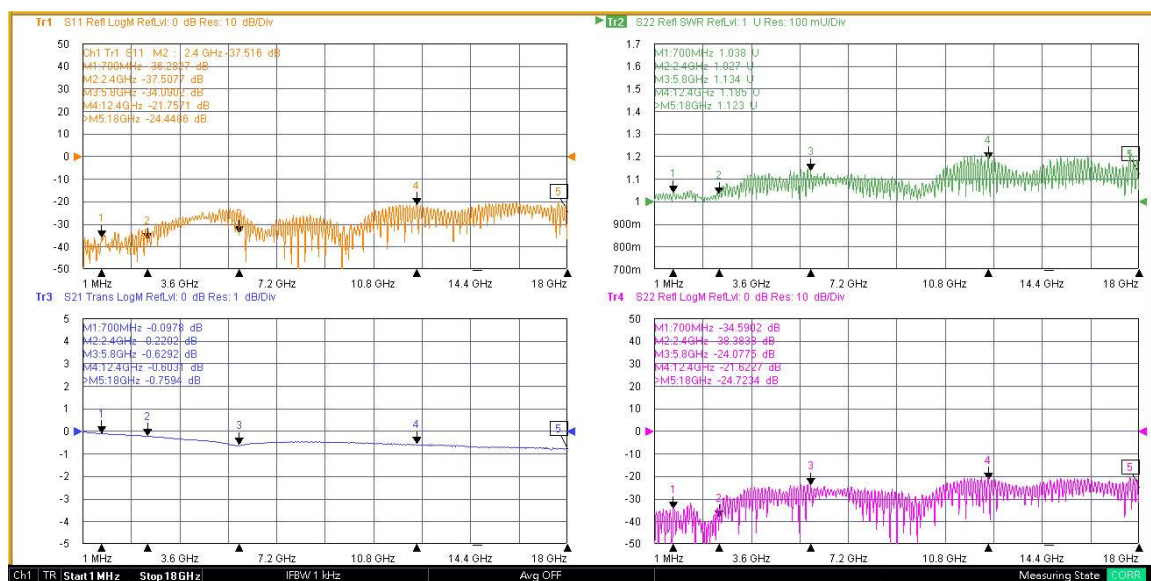
N(M)-SMA(M) 100cm
