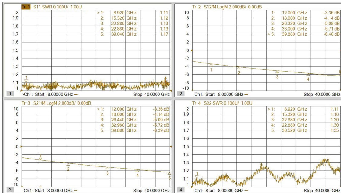
2.92mm(M)-SMPM(F)R/A 1.5M
