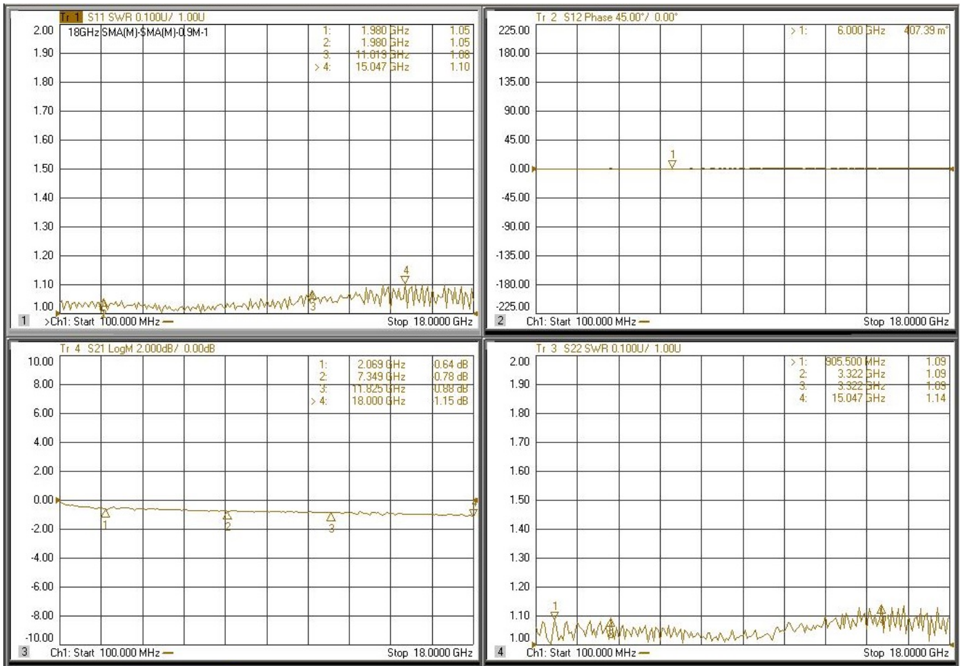
SMA(M)-SMA(M) 90cm
