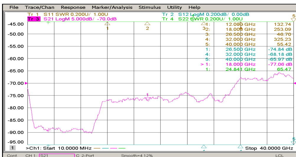
ISOLATION
