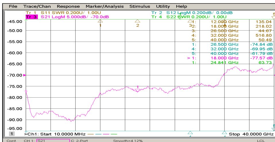
ISOLATION
