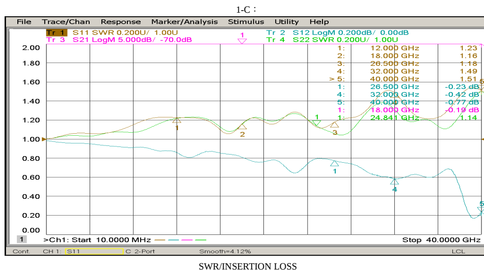
SWR/INSERTION LOSS
