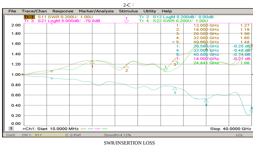
SWR/INSERTION LOSS
