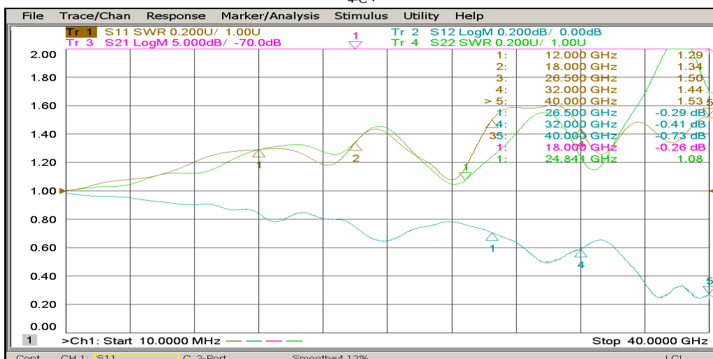
SWR/INSERTION LOSS
