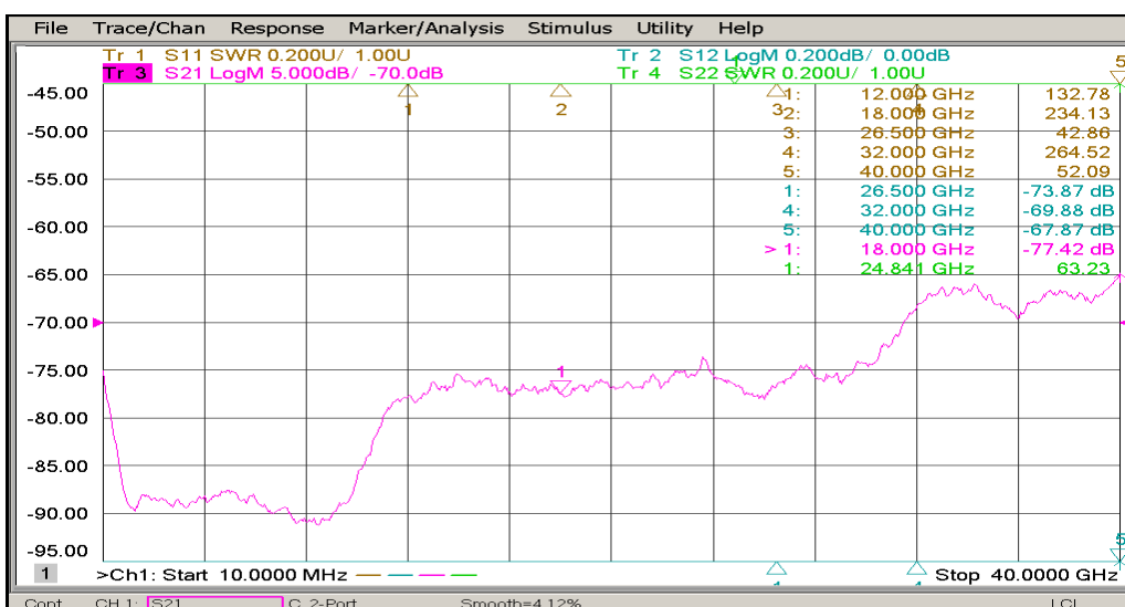
ISOLATION
