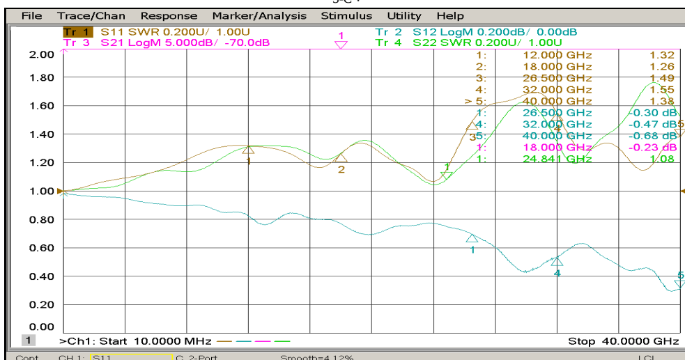
SWR/INSERTION LOSS
