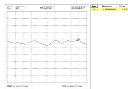
WR229 to N Female Waveguide Adapter
