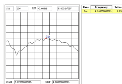
WR229 to N Male Waveguide Adapter
