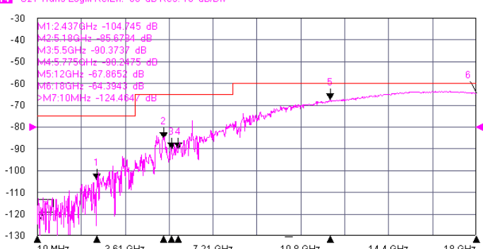
Port 7 Isolation
