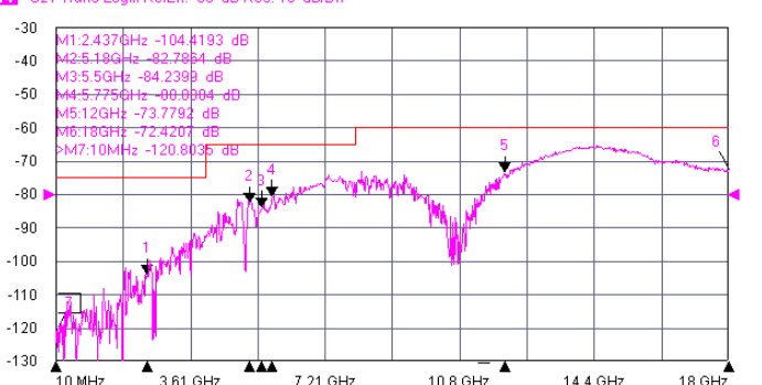
Port 6 Isolation
