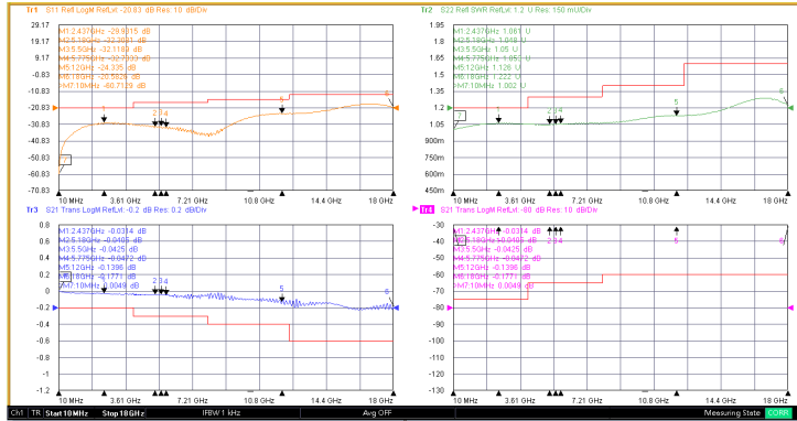
Port 3 Insertion Loss/VSWR
