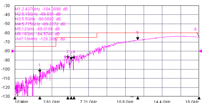
Port 8 Isolation
