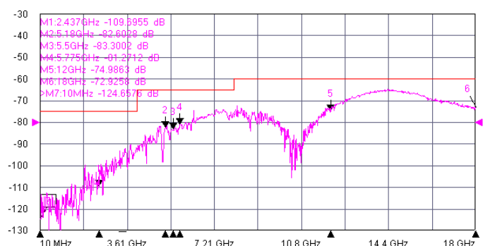
Port 5 Isolation
