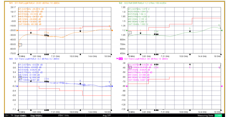
Port 6 Insertion Loss/VSWR
