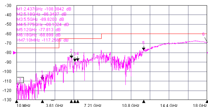
Port 3 Isolation
