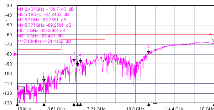
Port 4 Isolation
