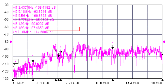
Port 8 Isolation
