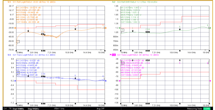
Port 4 Insertion Loss/VSWR
