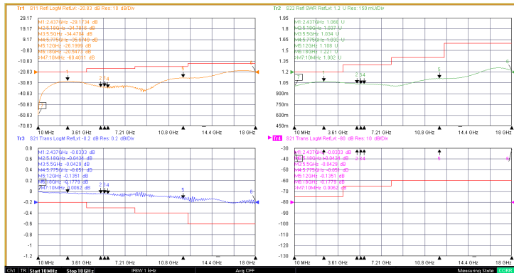
Port 5 Insertion Loss/VSWR
