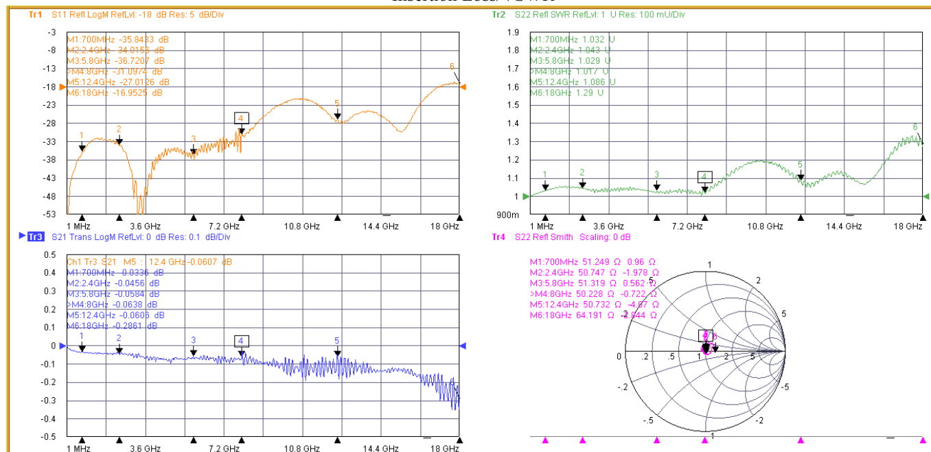
Insertion Loss/VSWR
