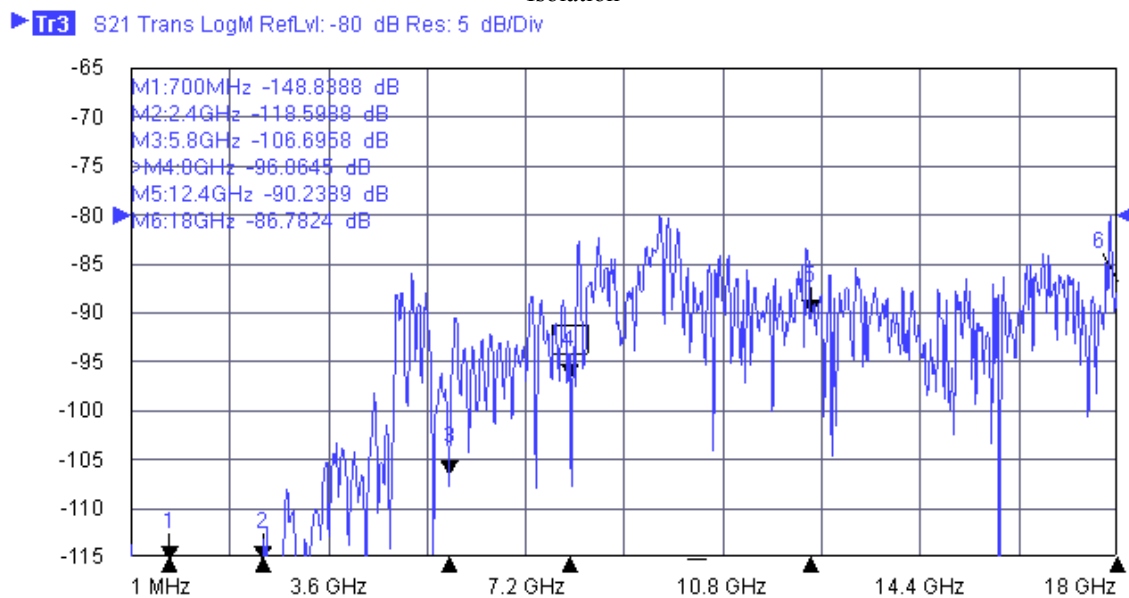
Isolation
