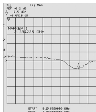
Insertion Loss
