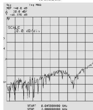
Isolation
