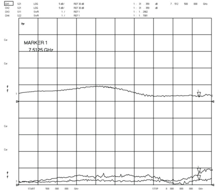
Gain/VSWR
